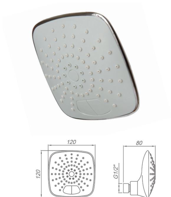
Square Shower Head 120mm
